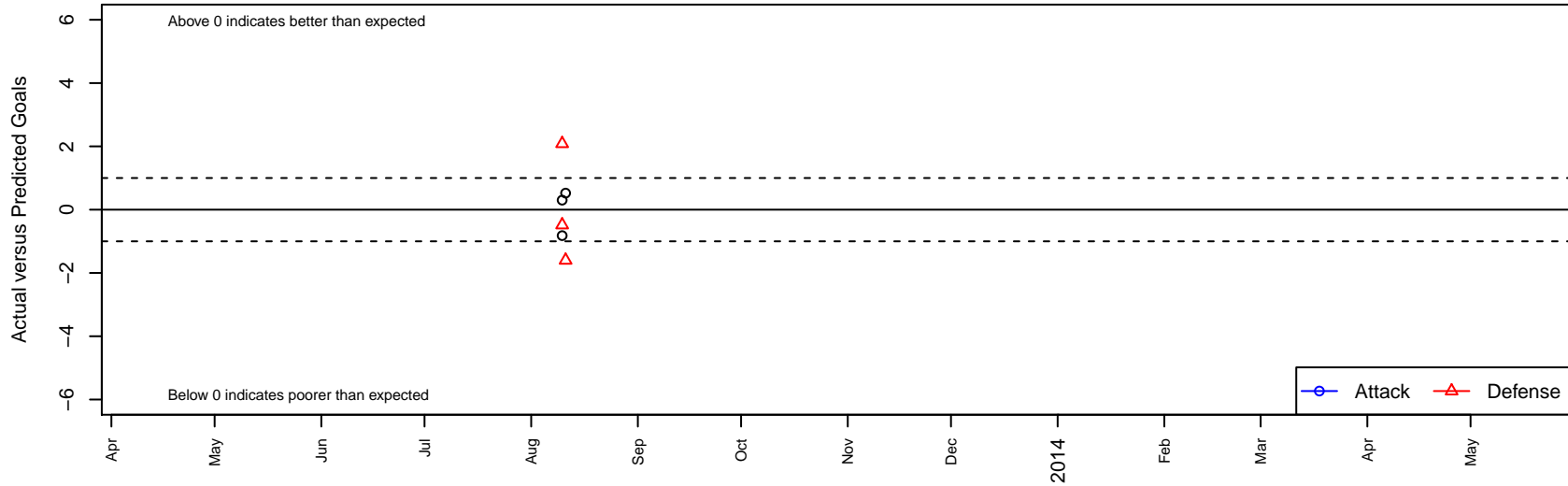
LASC Real Aztecas B02 Dots are actual minus expected GF (blue circles) and GA (red triangles). Blue line is smoothed change in attack strength. Red is smoothed change in defense strength.
